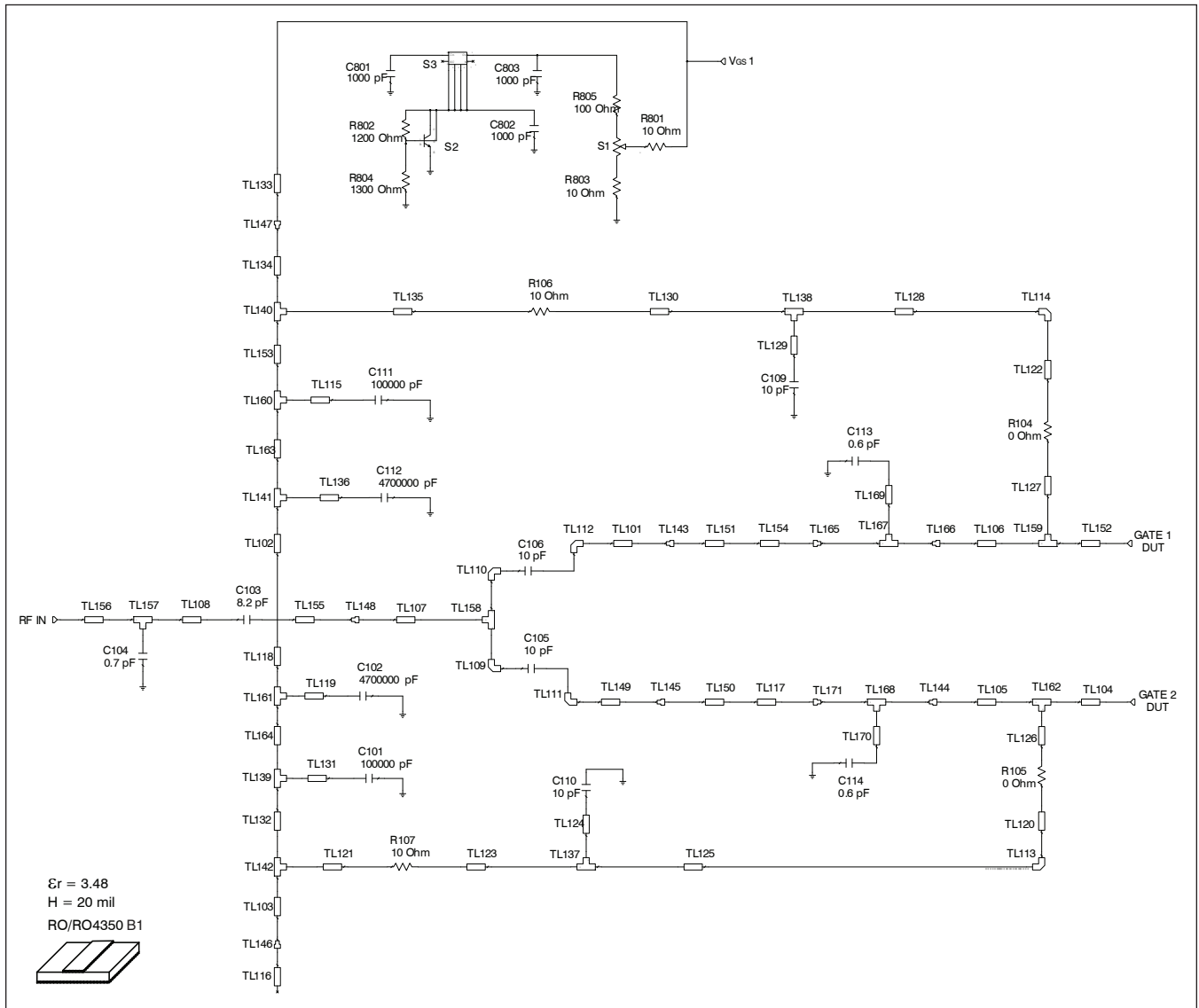
Reference circuit input schematic for f = 2170 \text{ MHz}
