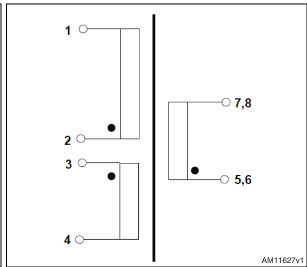
Figure 4. Transformer size and pin diagram electrical diagram
